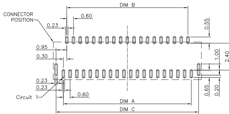
RECOMMENDED P.C.B PATTERN LAYOUT
